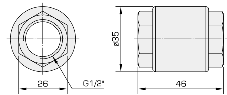
VC04 (G1/2")
